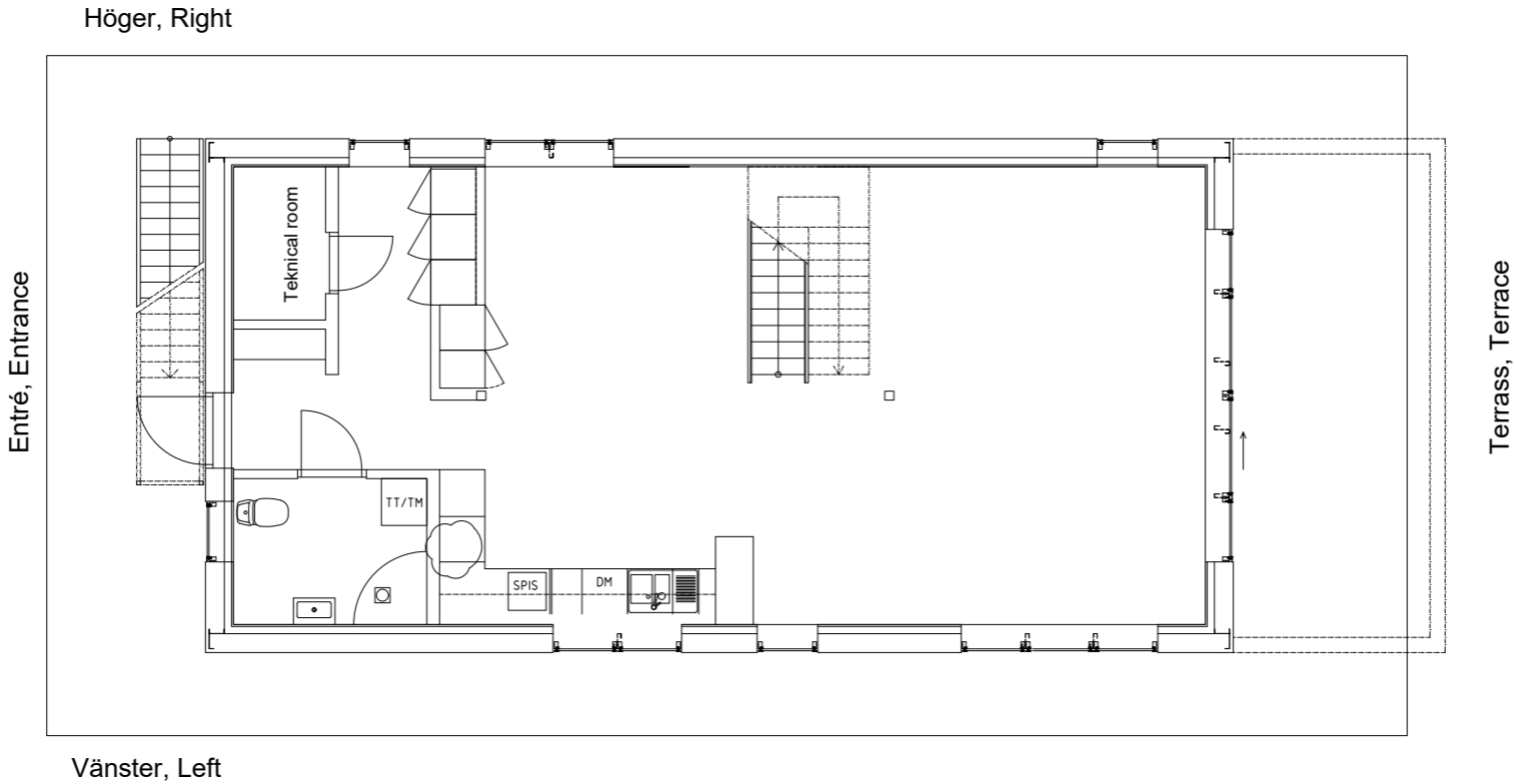
Plan 1, Entré, Entrance plan 78m 2
